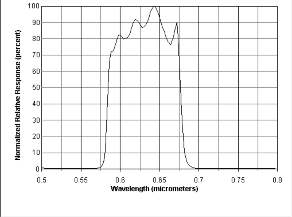
Figure D.2-1. Spectral Response Curve for NOAA-16 Channel 1.
