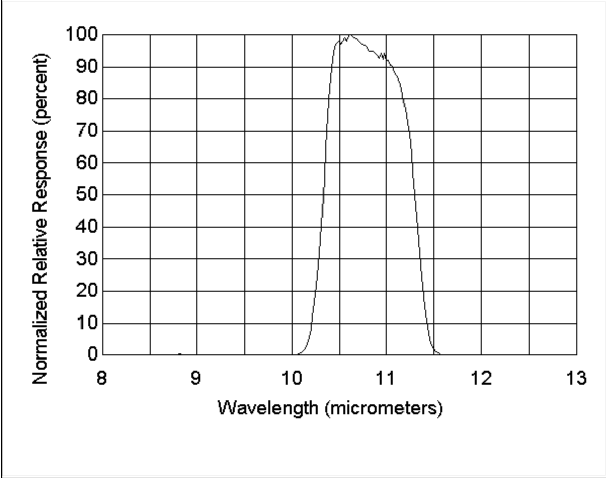
Figure D.4-5. Spectral Response Curve for NOAA-18 Channel 4.
