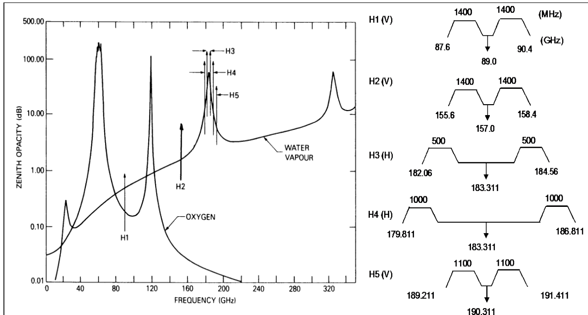
Figure 3.9.1-1. MHS Channels and Passband Arrangement
