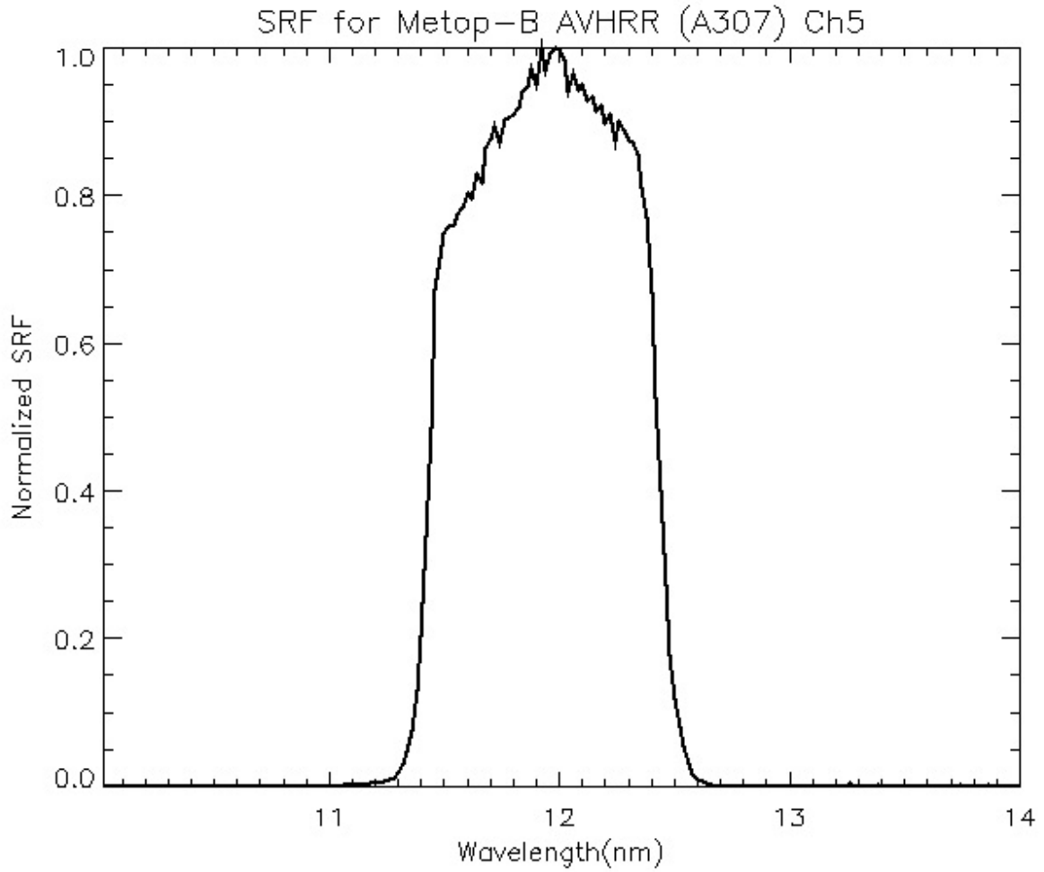
Figure D.7-6. Spectral Response Curve for MetOp-B Channel 5.
