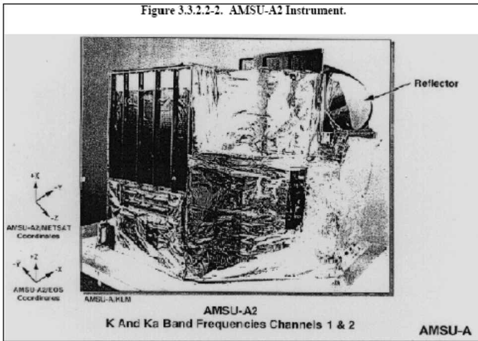
Figure 3.3.2.2-2 AMSU-A2 Instrument
