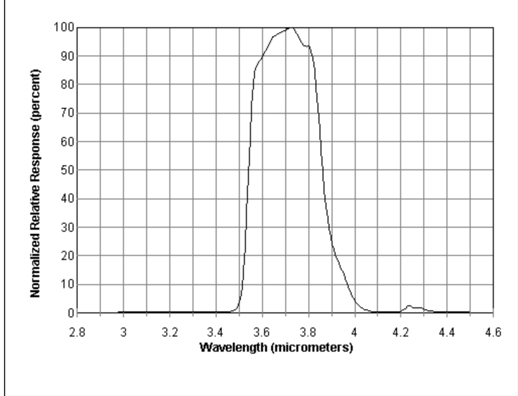
Figure D.2-4. Spectral Response Curve for NOAA-16 AVHRR/3 Channel 3B.
