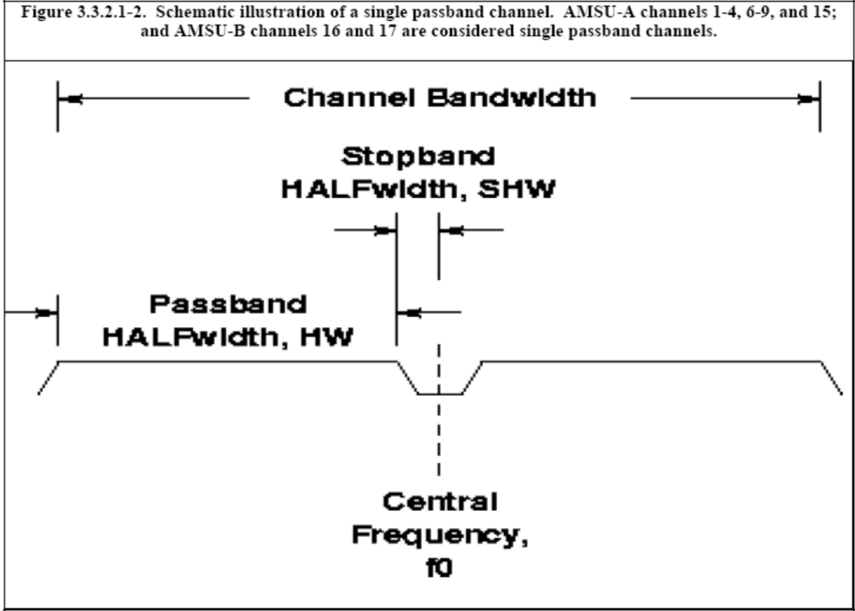
Figure 3.3.2.1-2. Schematic illustration of a single passband channel.
