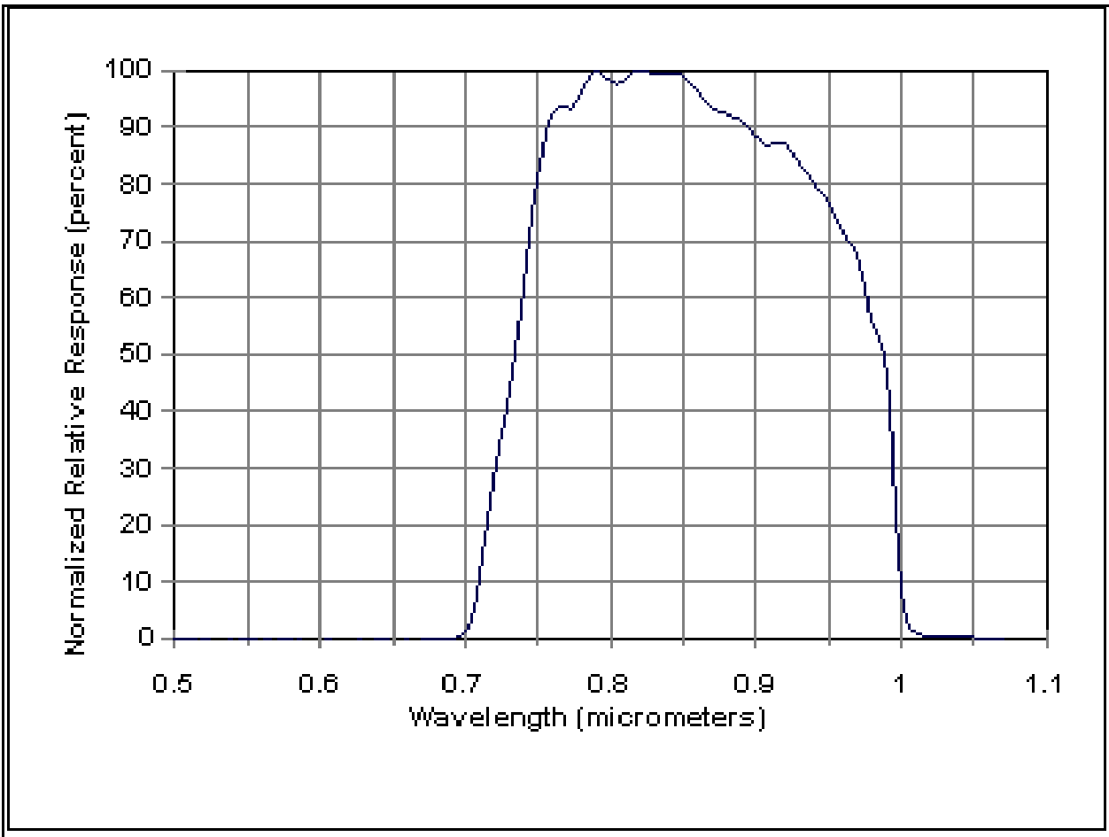
Figure D.3-2. Spectral Response Curve for NOAA-17 Channel 2
