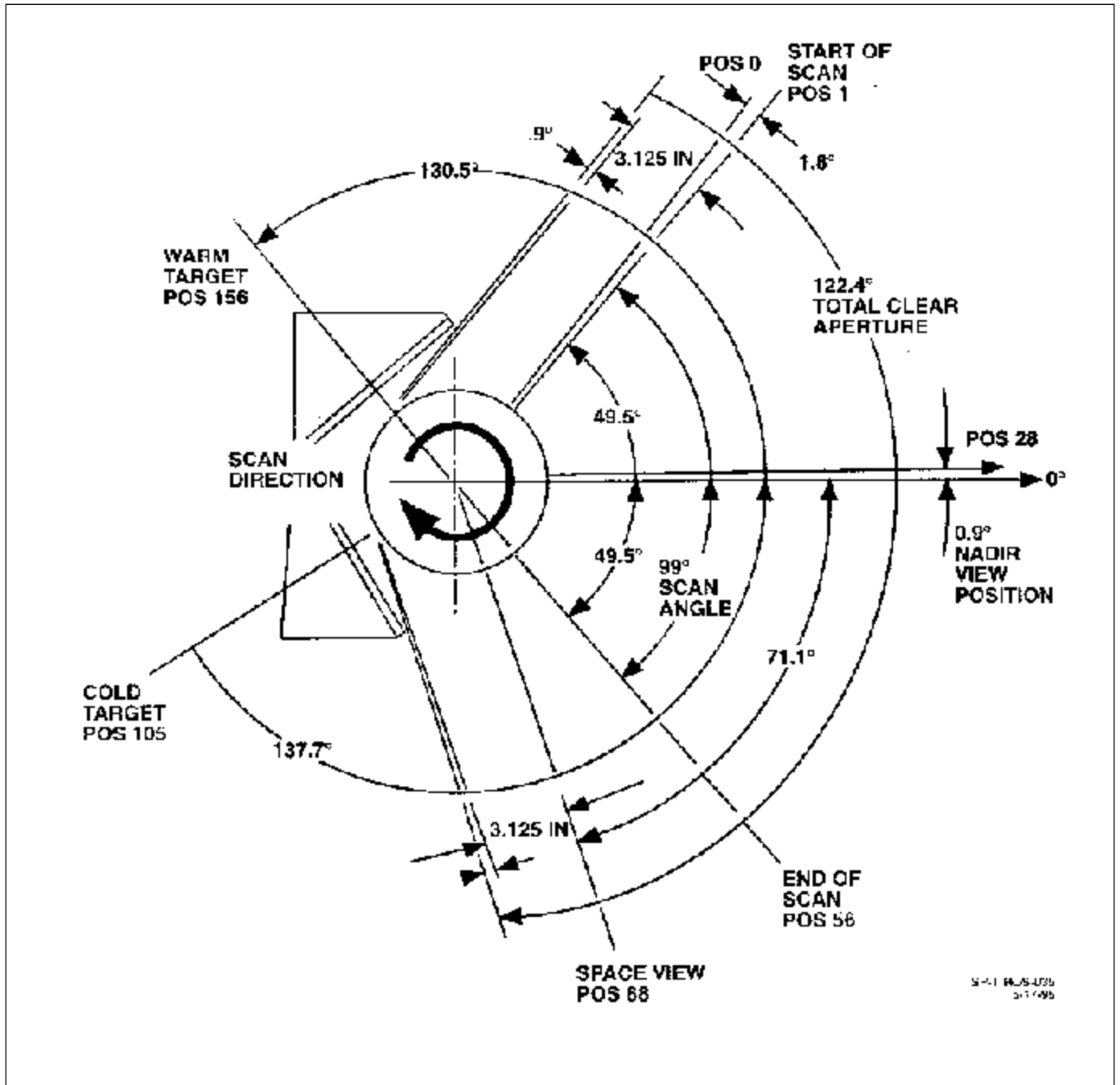
Figure J.2-1. Scan Angles for HIRS/3 and HIRS/4 Instruments
