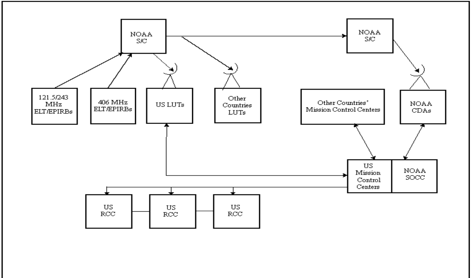
Figure 1.2.2.5-1. SARSAT Concept.
