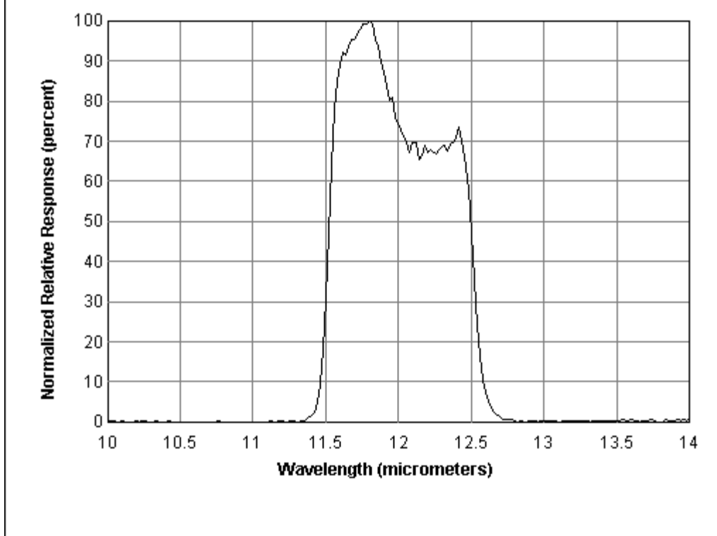
Figure D.2-6. Spectral Response Curve for NOAA-16 Channel 5.
