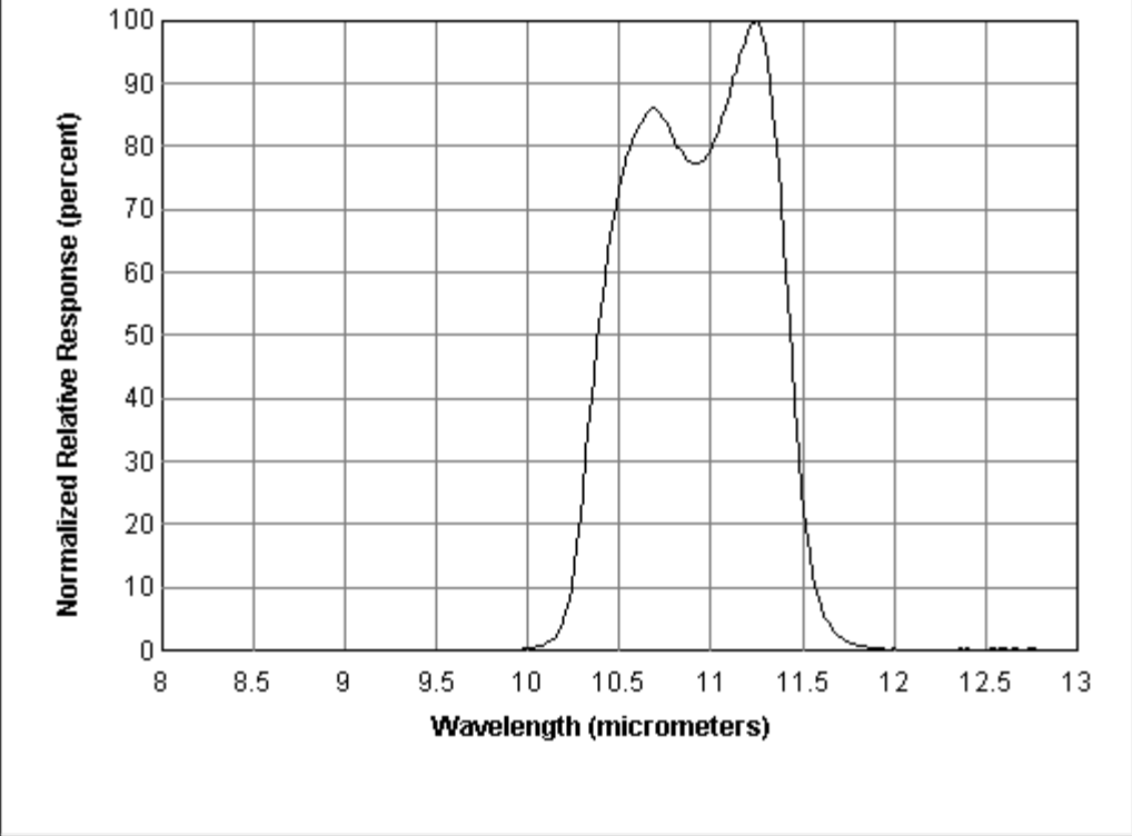
Figure D.2-5. Spectral Response Curve for NOAA-16 Channel 4.
