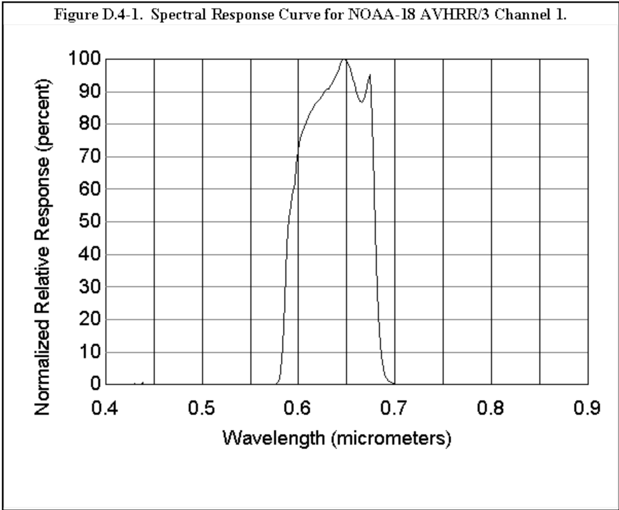
Figure D.4-1. Spectral Response Curve for NOAA-18 Channel 1.
