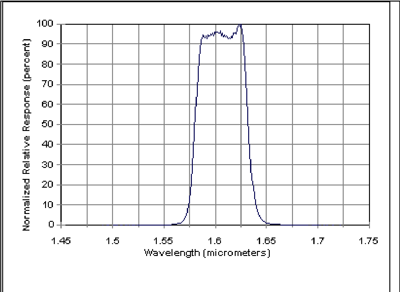
Figure D.3-3 Spectral Response Curve for NOAA-17 Channel 3A
