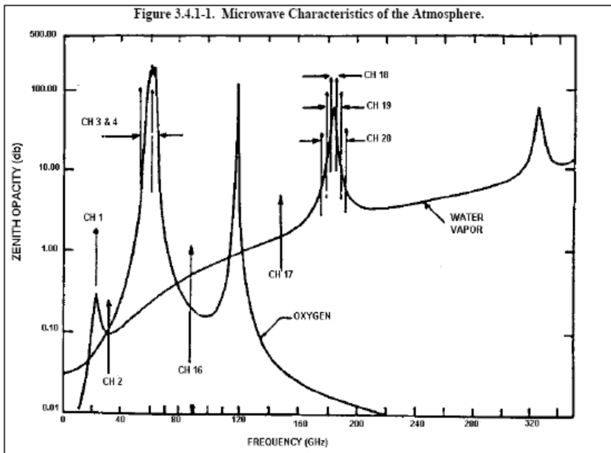
Figure 3.4.1-1 Microwave Characteristics of the Atmosphere.
