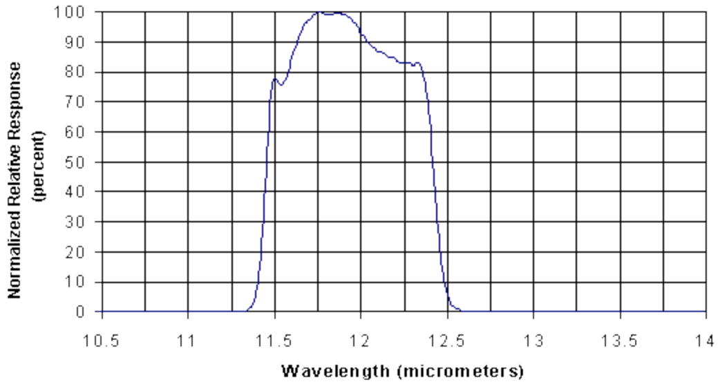
Figure D.1-6. Spectral Response Curve for NOAA-K AVHRR/3 Channel 5.
