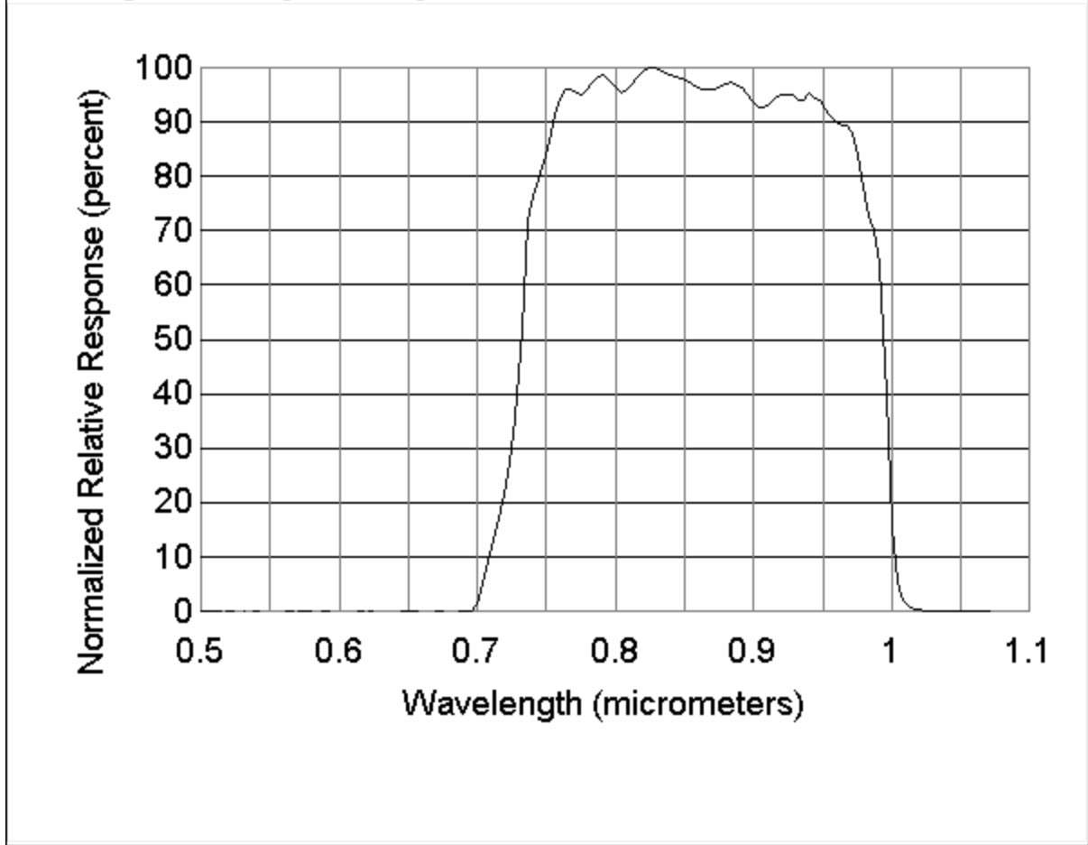
Figure D.4-2. Spectral Response Curve for NOAA-18 Channel 2.
