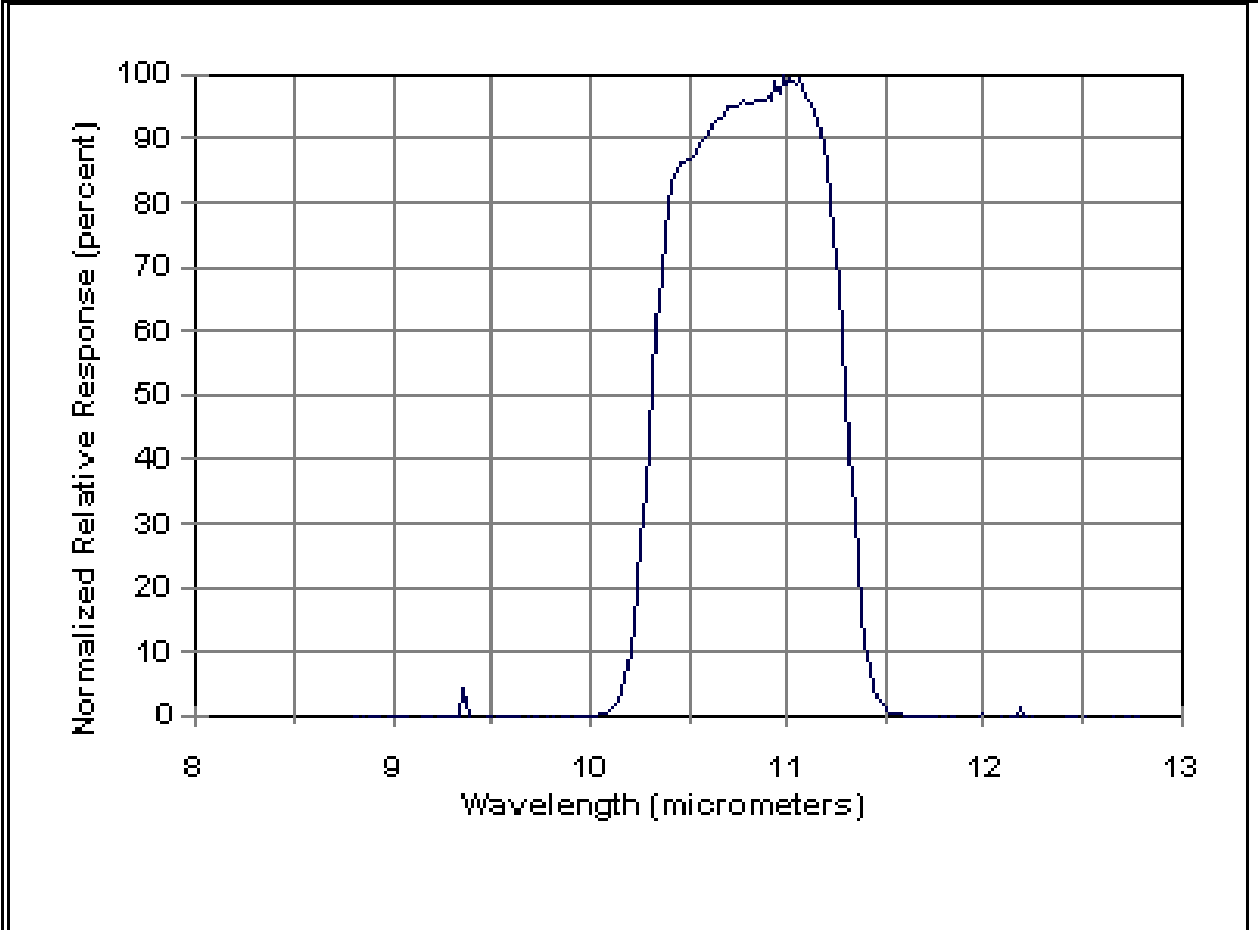
Figure D.3-5. Spectral Response Curve for NOAA-17 Channel 4
