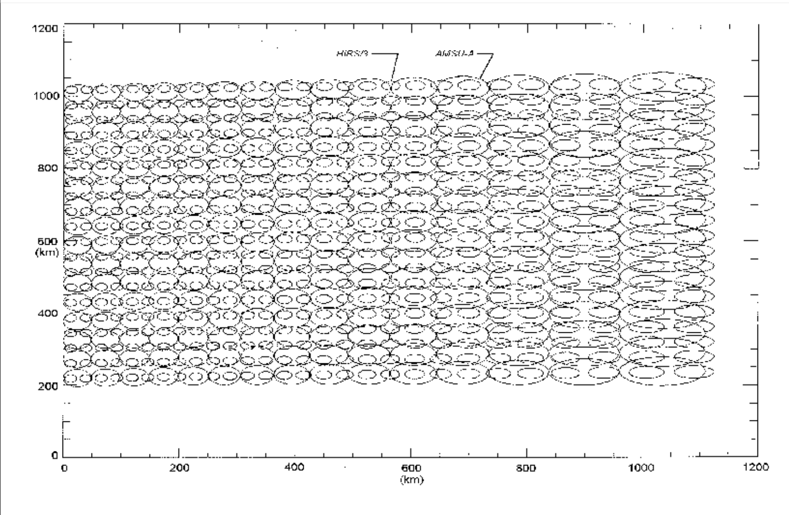
Figure J.2-2. Simulated Earth-surface footprints for HIRS/3 and AMSU-A (detail), half-scan.
