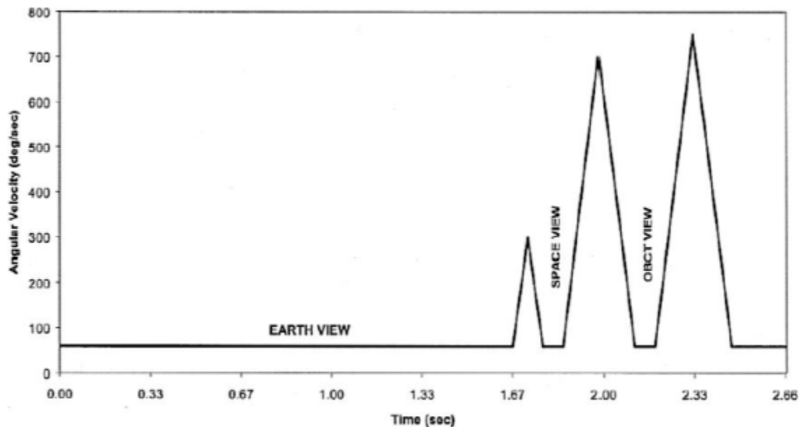
Figure J.3-6. MHS Scan Profile Velocity versus Time
