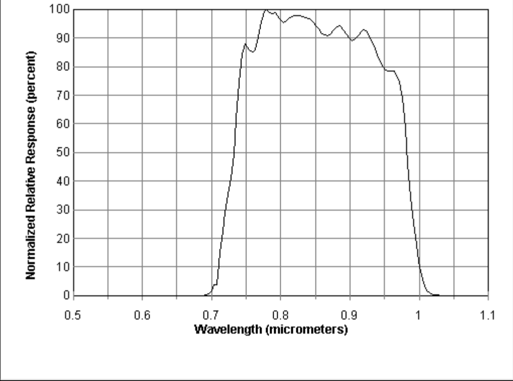
Figure D.2-1. Spectral Response Curve for NOAA-16 Channel 2.
